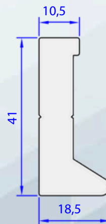
06785-00 1,180 Kg/m
