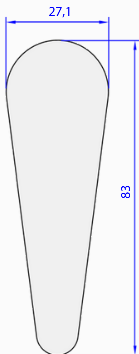
05095-00 4,238 kg/m
